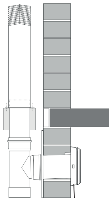
Wandlüfter AIRODOR Plus (#38014) *)
